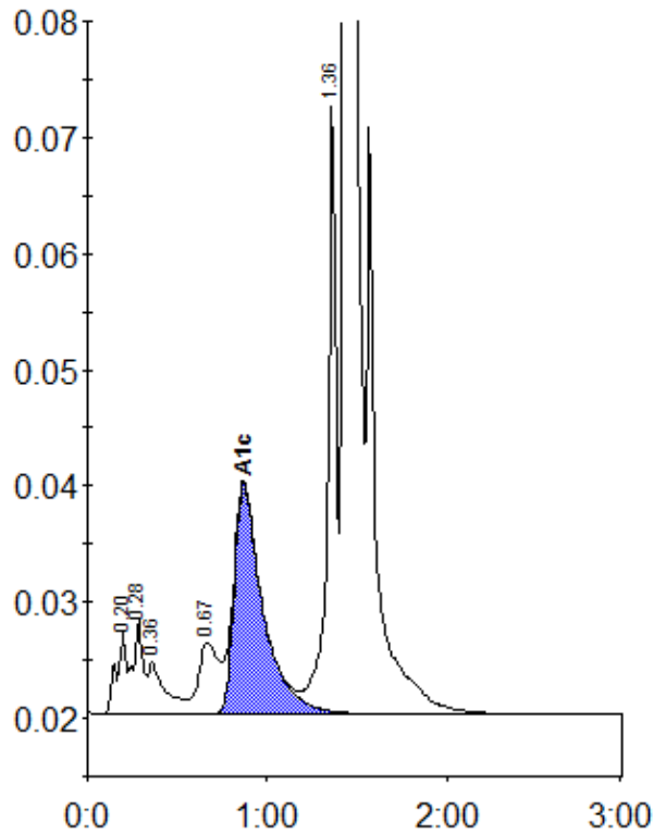
Peak table - ID: 10611677
